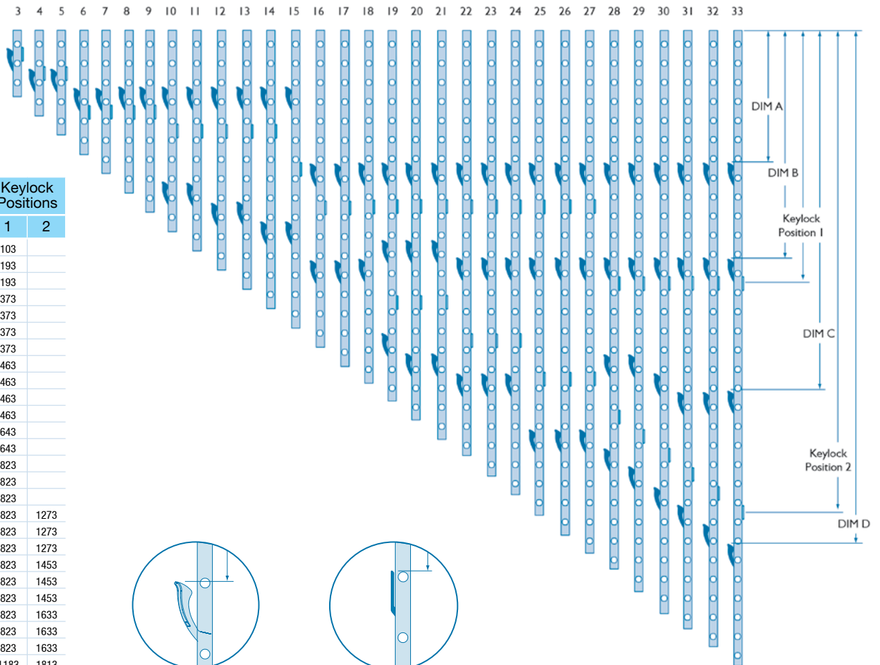
Standard Handle
