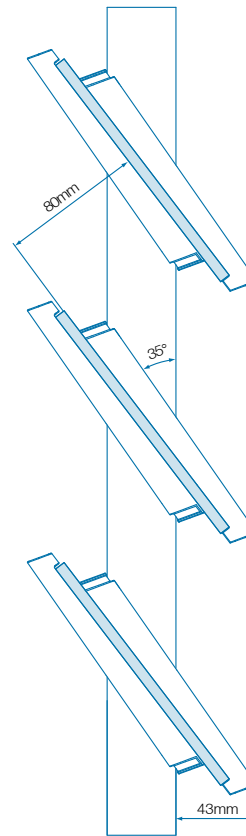
152mm Louvre 80mm Restricted Opening
