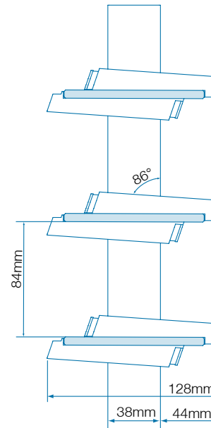
102mm Louvre Unrestricted Opening
